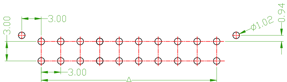
P. C. B LAYOUT
